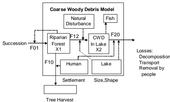
Fig. 1. Simulation model of CWD dynamics
