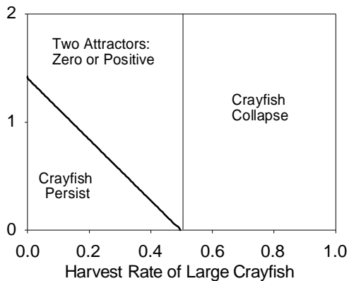
Fig. 3. Bifurcation diagram for model of crayfish population dynamics, showing different outcomes depending on harvest rate of large crayfish and predation by fishes on small crayfish. Dynamics were generated by A(t+1) = (1 - k) A(t) + f A(t) \{1 - m A(t) - [c / (1 + A(t)^q)]\} where A is the adult crayfish population, k is mortality of adults from harvest, f is fecundity, m is density-dependent mortality, c is the predation coefficient for fishes consuming juvenile crayfish. Parameter values: f=0.5 , m=0.01 , q=4 .
