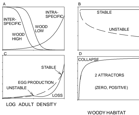
Fig. 2. Dependence of a piscivore driven by consumption of its juveniles by other species. A. Piscivore mortality rate from interspecific predation and intraspecific causes. Interspecific predation decreases as woody habitat increases. B. Stable and unstable densities of piscivore adults versus woody habitat. C. Egg production and total mortality of juvenile piscivores versus adult piscivore density, showing stable and unstable intersections. D. Bifurcation diagram for mortality rate of adults due to fishing and woody habitat, showing boundary between the zone of piscivore collapse and the zone where piscivores either persist stably or collapse, depending on initial conditions. Dynamics are generated by
